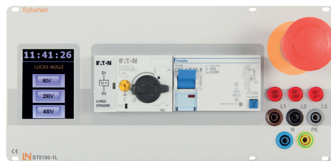
Lab supply panel for student work station featuring touch-panel client, order no. ST8100-1C
