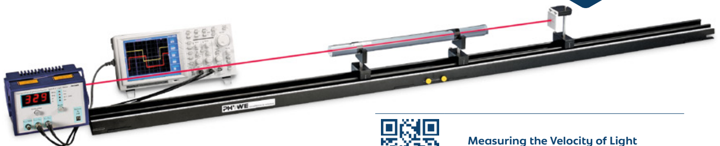
Measuring the Velocity of Light Art. no. P2210101
