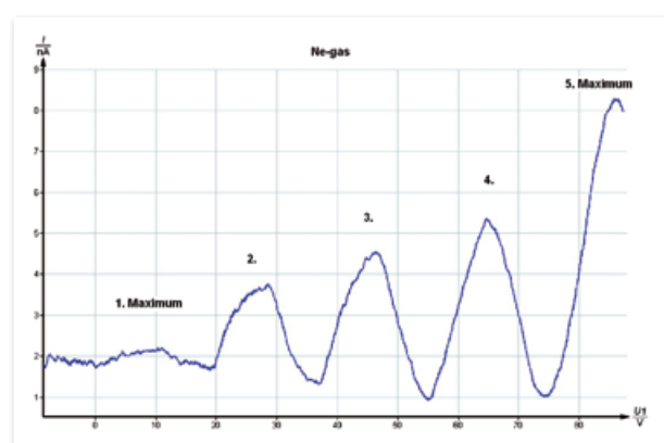
Example of a Franck-Hertz curve for Ne-gas
