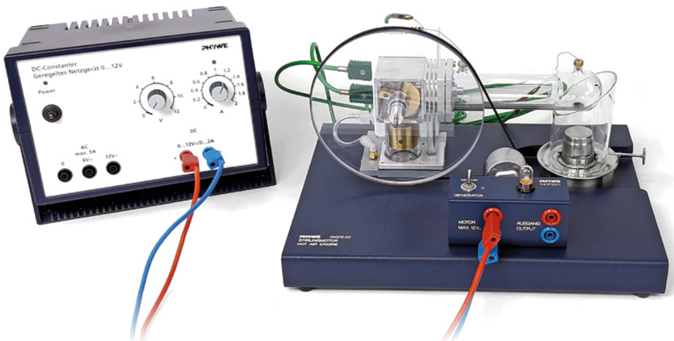
Stirling Engine with measureLAB Art. no. P2360467
