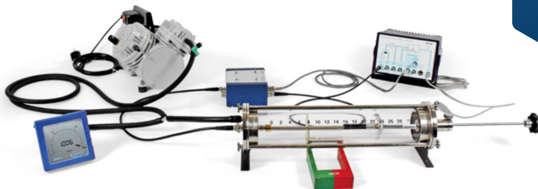
Rutherford Experiment Art. no. P2522115
